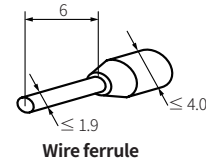
Wire ferrule
