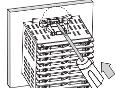
Flathead screwdriver
